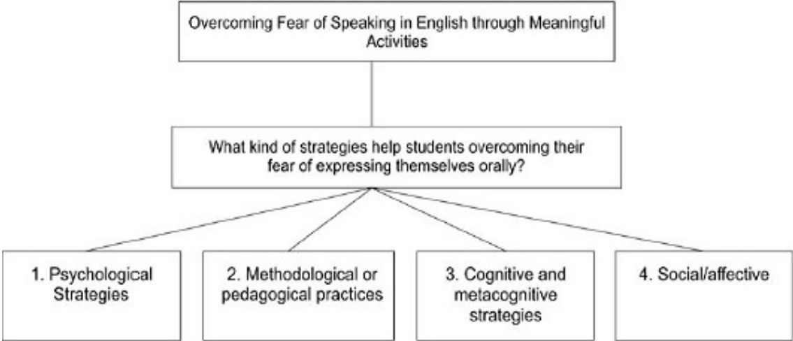
Diagram 3. Categories found in the data analysis.
